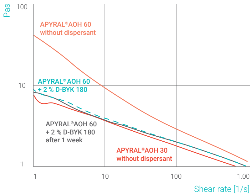
Figure 5: Viscosity as a function of shear rate for edge-coating slurries. Influence of boehmite choice (APYRAL® AOH 30 vs. APYRAL® AOH 60), effect of dispersant (+2 % D-BYK) and slurry ageing (after 1 week) are demonstrated.
