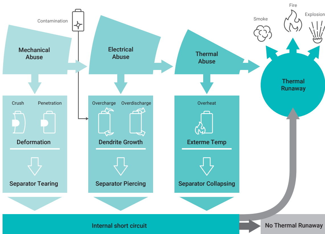
Figure 1: Abuse conditions leading to thermal runaway.
