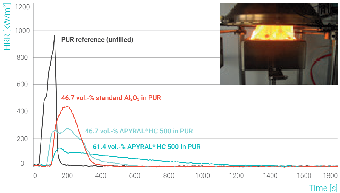
Figure 18: Cone measurement of PUR. Heat release rate of unfilled PUR in comparison with APYRAL® HC 500 and standard Al 2 O 3 filled PUR.
