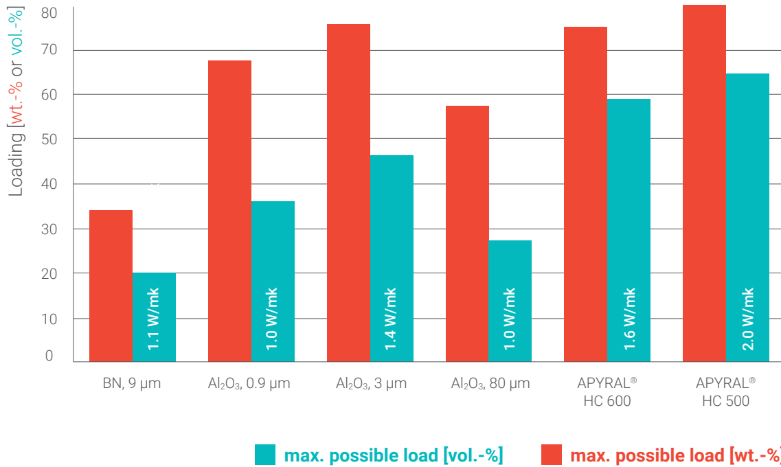
Figure 13: TC of APYRAL ® HC in comparison to calcined alumina, and BN in UP-resin at 22 °C (Hot Disk method).
