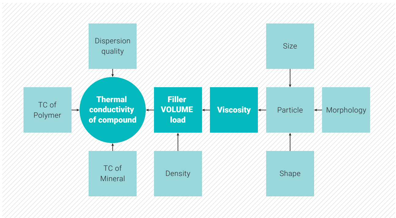
Figure 7: Important parameters to influence the thermal conductivity of a polymer compound.
