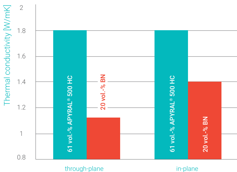
Figure 12: Thermal conductivity of an UP resin filled with BN or APYRAL® 500 HC, measured in- and through-plane.
