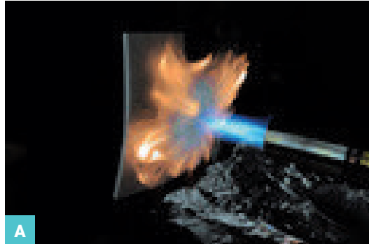
Figure 19: Compound plate during torch testing (A). UP resin filled with simple flame retardant (B) and Nabaltec's proprietary filler system ACTILOX® HTB (C) after testing.
