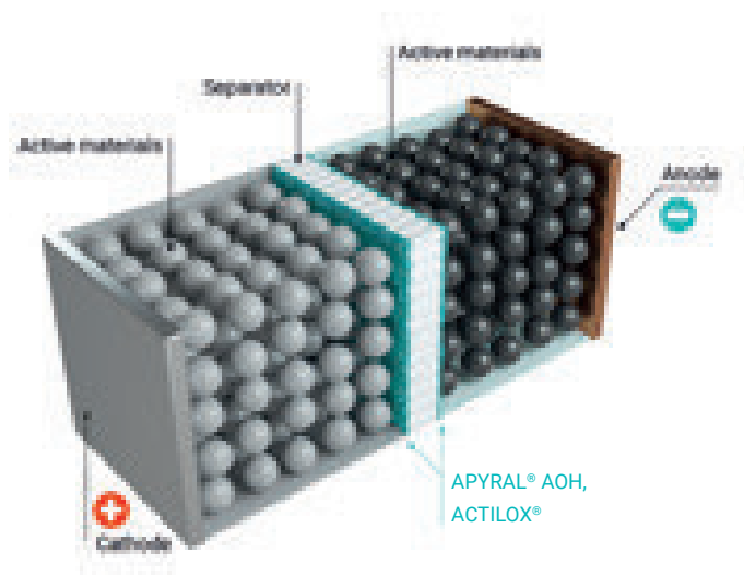
Figure 2: Three-dimensional structure illustration of a Lithium ion battery cell.
