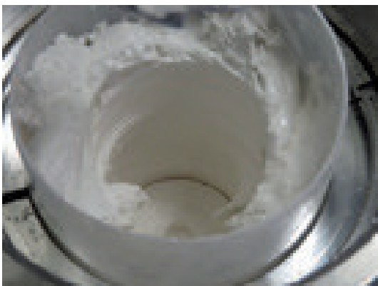
Figure 11: Aborted experiment trying to disperse 27 vol.-% of BN in UP-resin. All material clogs to the wall while the dissolver blade (not shown) is mixing only air.
