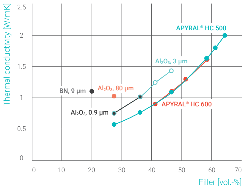
Figure 9: Relative viscosity of APYRAL® HC in comparison to calcined Al_2O_3 , and BN in UP resin at shear rate 10\ s^{-1} at 22\ ^\circ C (above) and the corresponding TC values obtained by Hot Disk method after curing (below).
