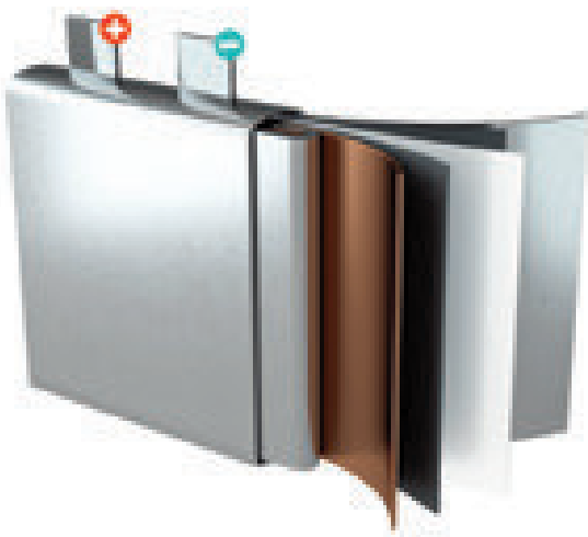
Figure 2: Three-dimensional structure illustration of a Lithium ion battery cell.
